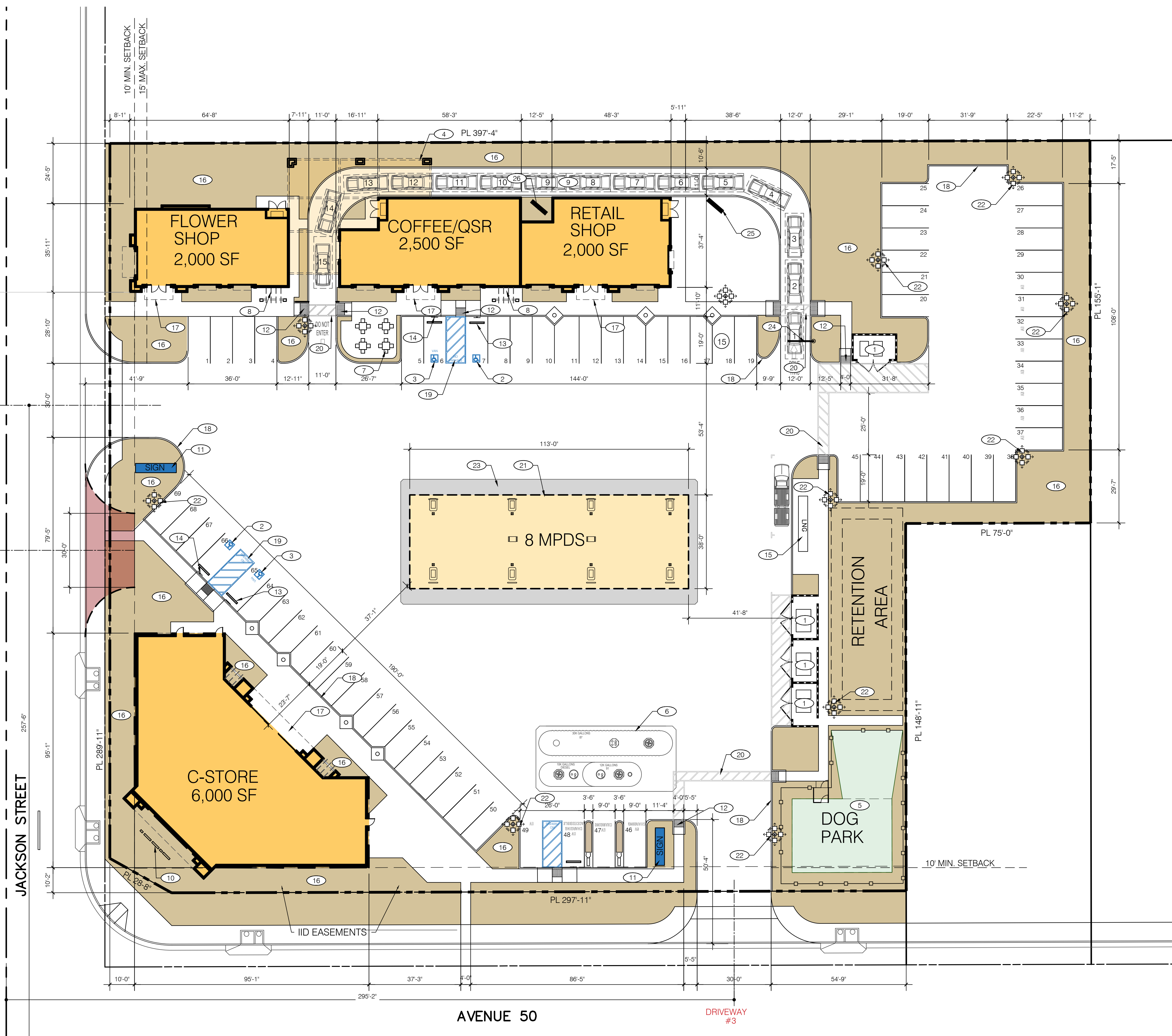
SITE PLAN SCALE: 1"=20'-0" 2.48 AC
