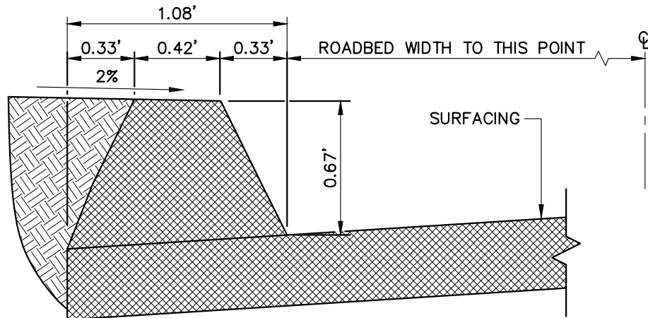
8" A.C. DIKE NOT TO SCALE
