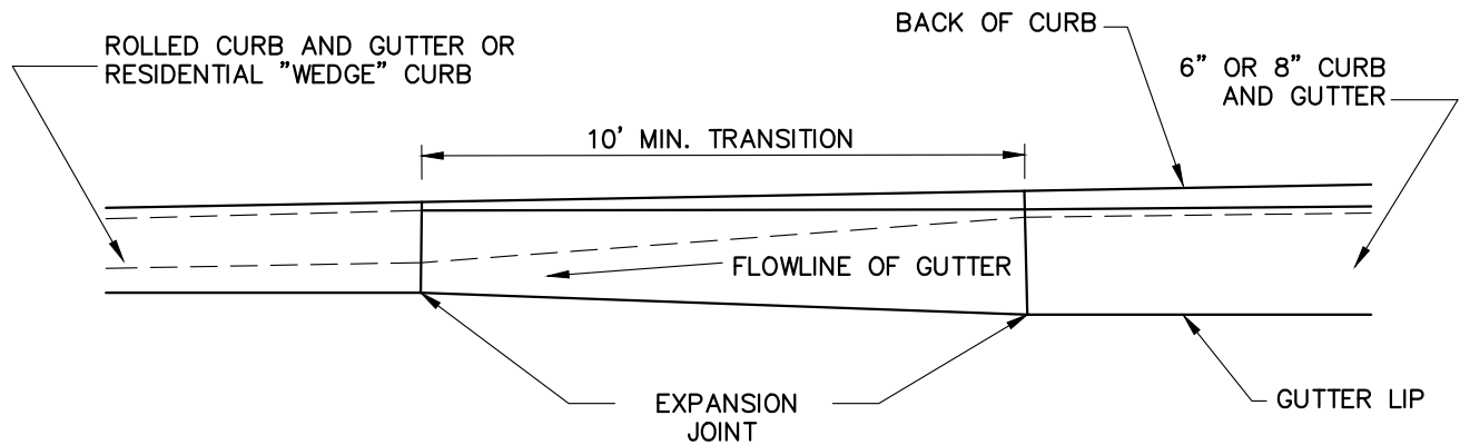
PLAN VIEW
