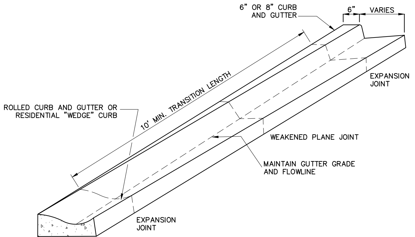
ISOMETRIC VIEW
